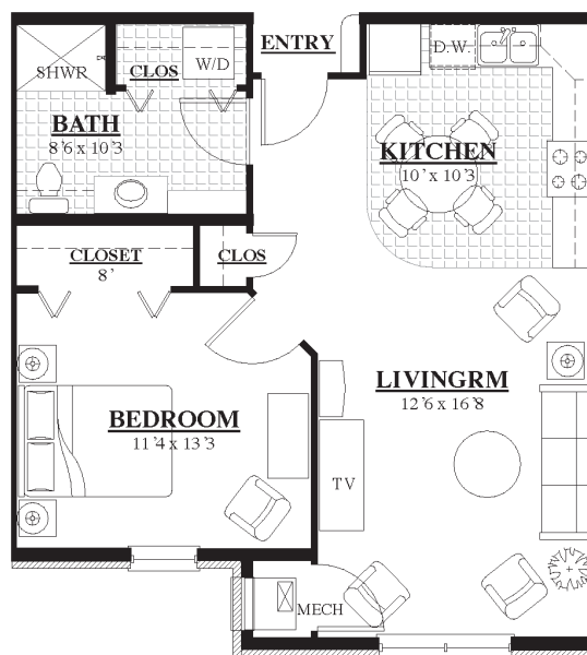
1 bedroom - floorplan B Core 706 Square Feet
