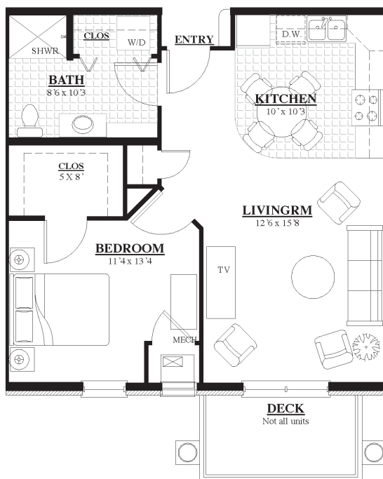
1 bedroom - floorplan A 694 Square Feet
